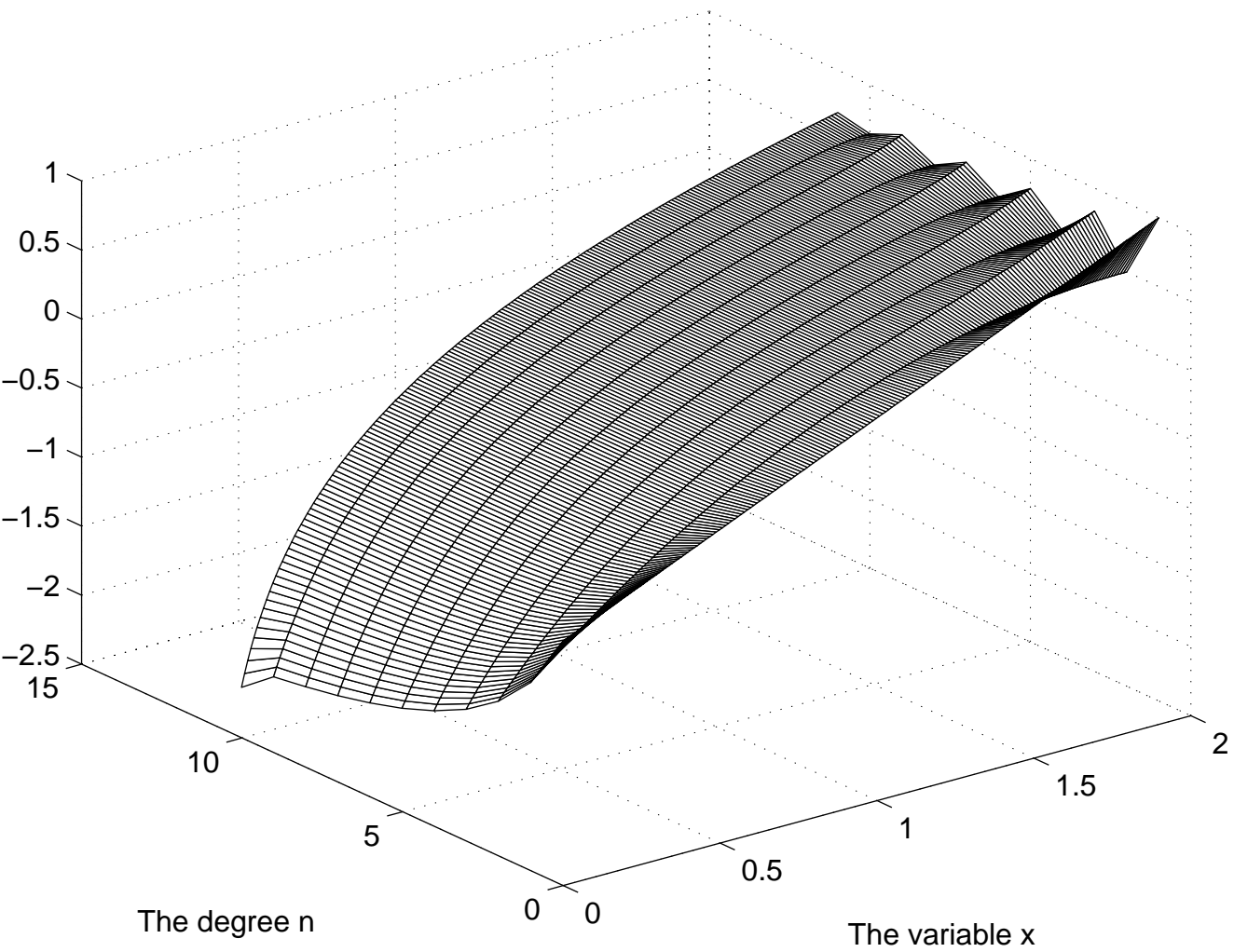
Graphs of Taylor polynomial for \log(x)
