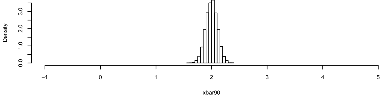
Histogram of xbar90
