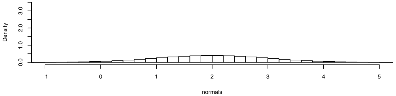
Histogram of normals
