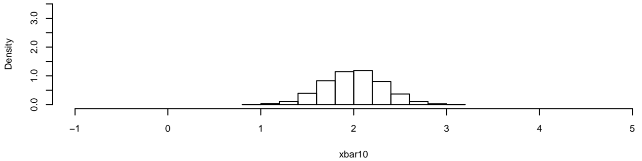
Histogram of xbar10
