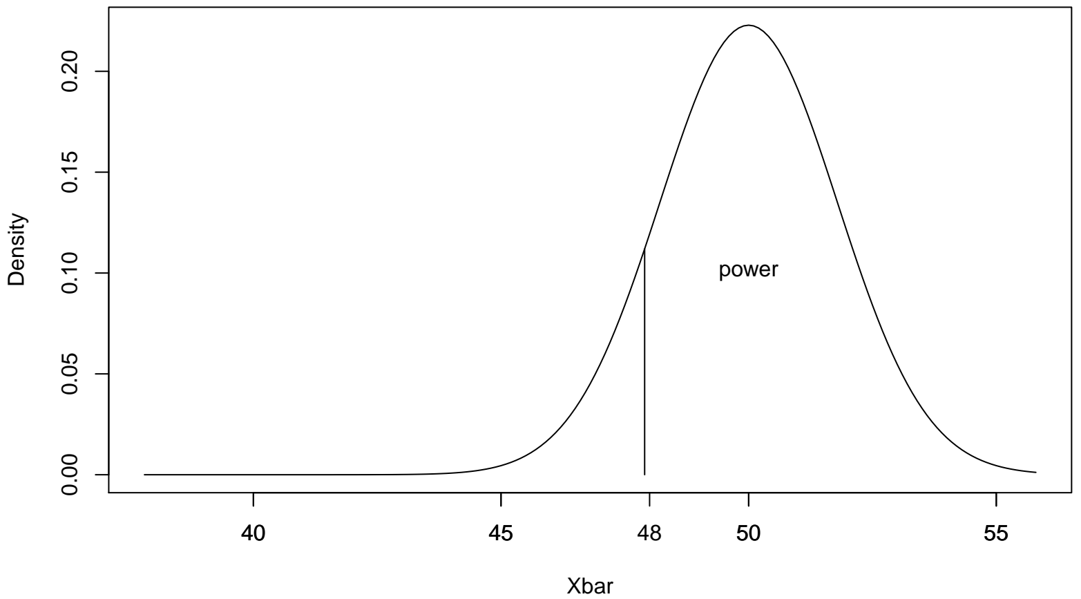
Sampling distribution of Xbar under H A , mu = 50
