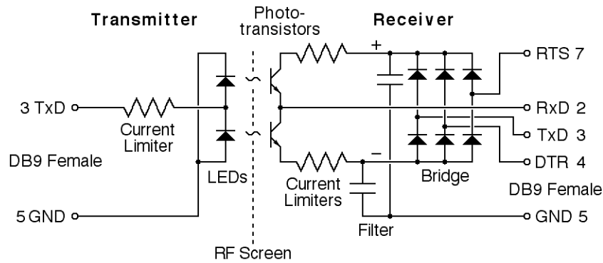
Figure 1: Schematic of the data diode.
