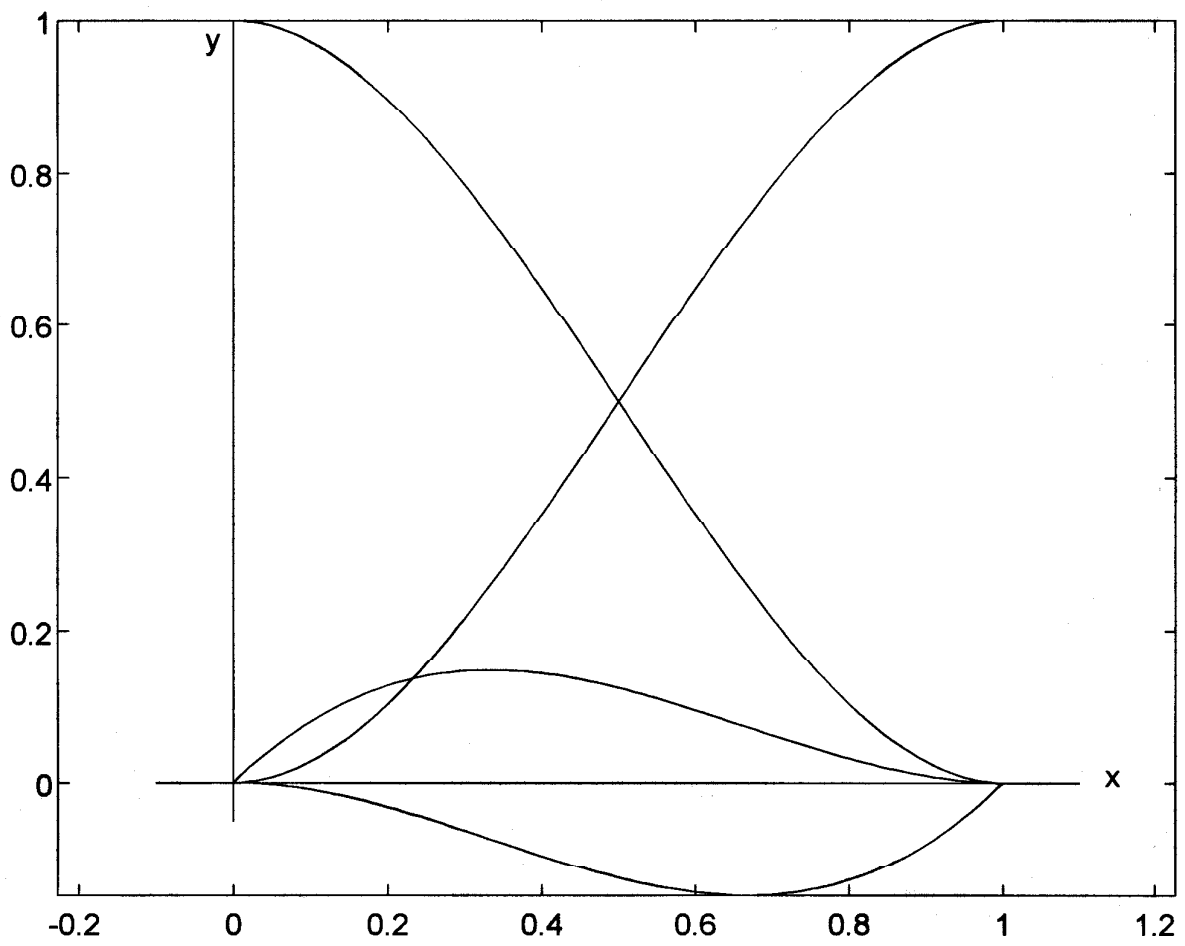
2-point Hermite interpolation basis functions
